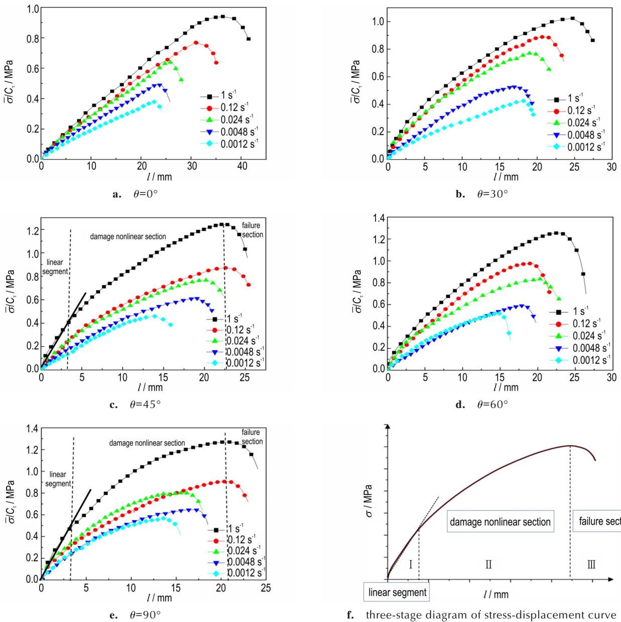
图4 不同拉剪角度和不同应变率下NEPE推进剂拉剪复合加载应力-位移曲线和应力-位移曲线三阶段图 Fig.4 Stress-displacement curves of NEPE propellant under combined tensile-shear loadings with different tensile-shear angles and different strain rates, and the three-stage diagram of stress-displacement curve
