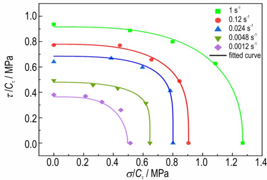
图6 不同应变率加载条件 NEPE 推进剂极限承载力散点图及拟合曲线 Fig.6 Scatter diagram and fitting curves of the ultimate bearing capacities of NEPE propellant with different strain-rate loading conditions
