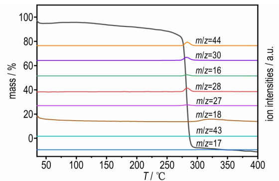
a. TG-MS curves of HMX
