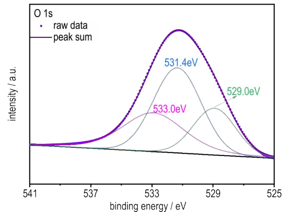
d. O 1s core level spectrum of the Fe@CNTs
