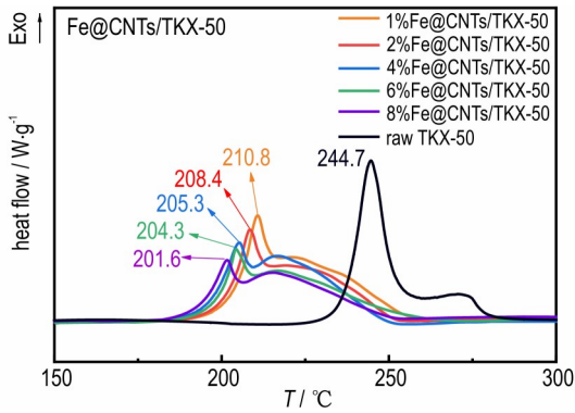
图7 不同含量Fe@CNTs催化TKX-50的DSC曲线( \beta=10\text{ °C}\cdot\text{min}^{-1} ) Fig.7 DSC curves of TKX-50 catalyzed by different contents of Fe@CNTs( \beta=10\text{ °C}\cdot\text{min}^{-1} )
