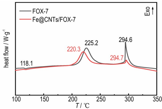
a. DSC curves of FOX-7 and Fe@CNTs/FOX-7
