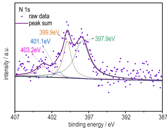
c. N 1s core level spectrum of the Fe@CNTs
