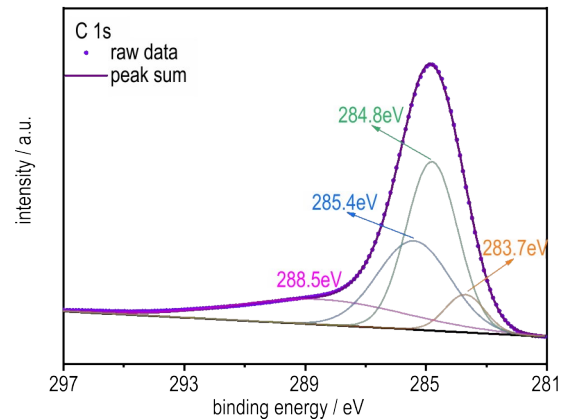
b. C 1s core level spectrum of the Fe@CNTs
