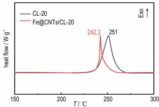
c. DSC curves of CL-20 and Fe@CNTs/CL-20
