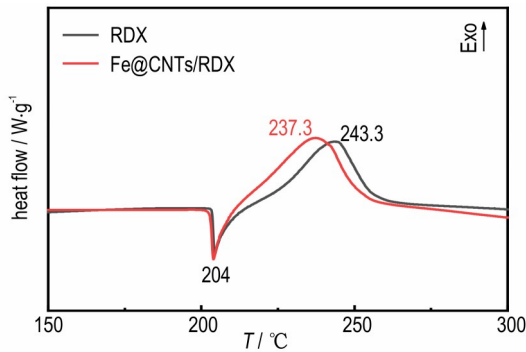
b. DSC curves of RDX and Fe@CNTs/RDX
