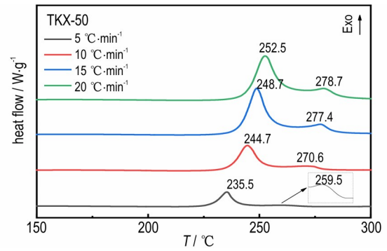
a. DSC curves of TKX-50
