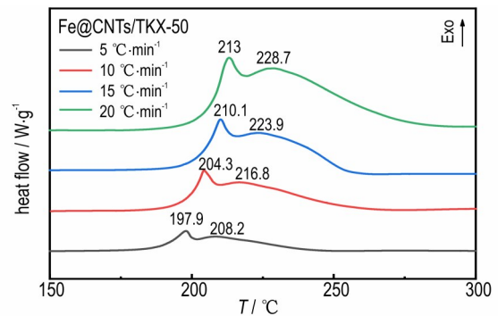
b. DSC curves of Fe@CNTs/TKX-50
