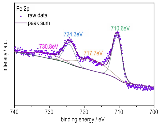
a. Fe 2p core level spectrum of the Fe@CNTs
