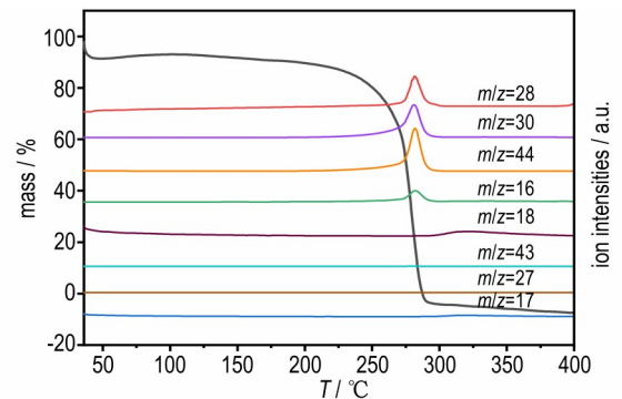
b. TG-MS curves of Fe@CNTs/HMX
