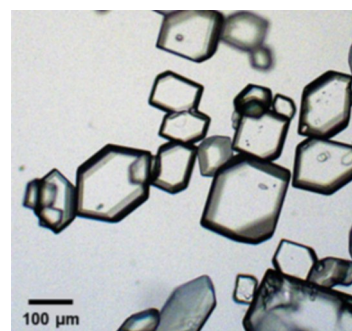
c. ADN/PDO cocrystal
