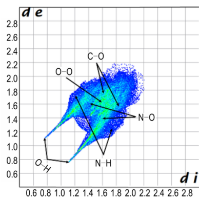
c. 2D fingerprint plot
