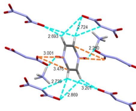
b. intermolecular interaction of ADN/PDO cocrystal
