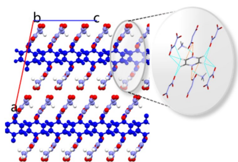
a. packing type diagram
