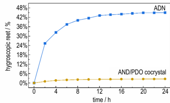
b. hygroscopicity curves
