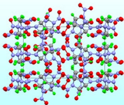
The structure of \beta -CL-20/HMX cocrystal
