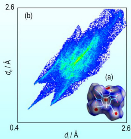
Hirshfeld surface (a) and fingerprint plot (b) of CL-20 molecule in \beta -CL-20/HMX cocrystal
