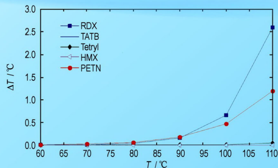
relationship between temperature deviation and test temperature
