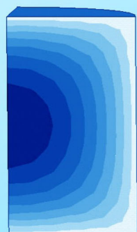
internal temperature field of RDX cylinder at 100 °C
