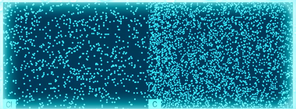
distribution of elements Cl and C for HMX/AP/EP
