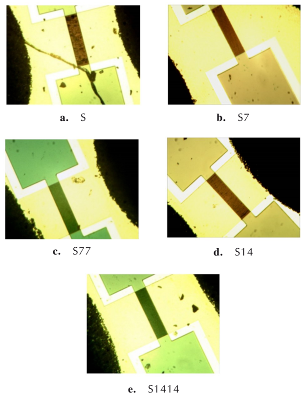
图11 静电放电后SCB火工品桥区显微照片 Fig.11 Micrograph of SCB initiator bridge area after electrostatic discharge
