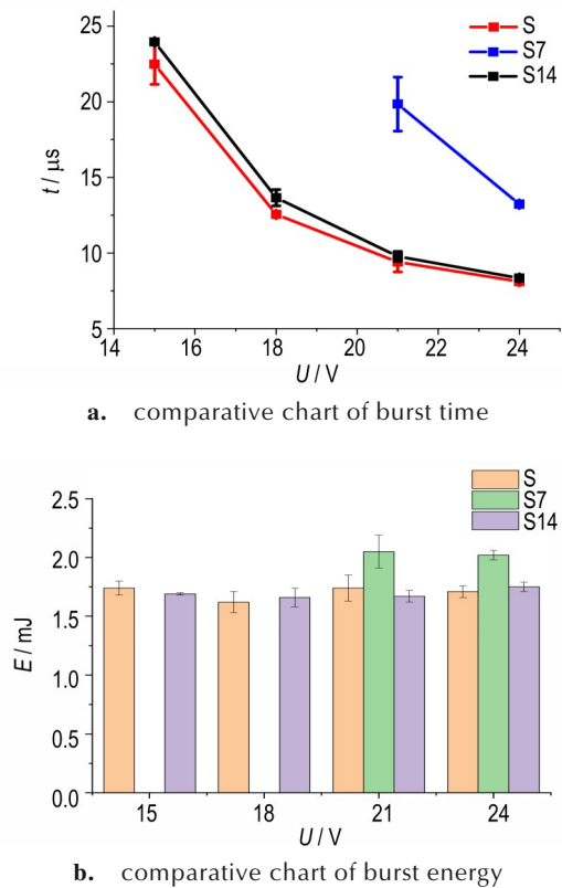
图10 S、S7和S14型样品爆发时间和爆发能量对比图 Fig.10 Comparison of burst time and burst energy for S, S7, and S14 samples
