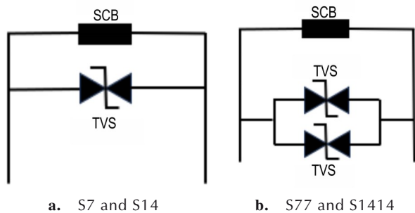
图 3 TVS 二极管与 SCB 火工品并联等效电路图 Fig.3 Circuit diagram of the equivalent parallel connection of TVS diode and SCB initiator device
