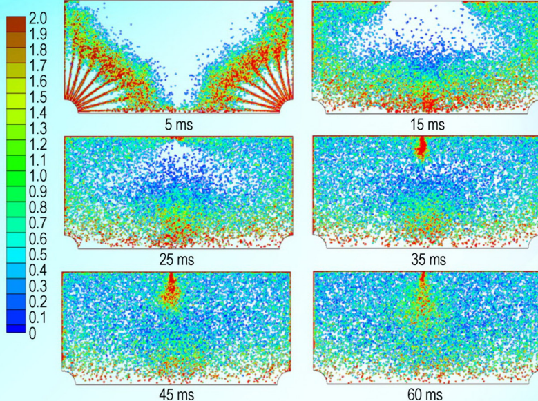
turbulence kinetic energy in chamber at different time
