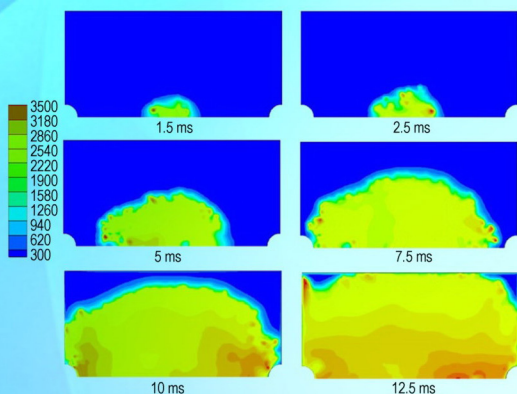
concentration profile of aluminum dust in chamber at different time
