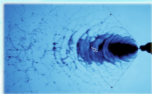
atomization image ( v_{jet} = 22.14 \text{ m}\cdot\text{s}^{-1} , \beta = 100^\circ )
