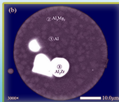
Surface morphology of \text{Al}_{78}\text{Mg}_{20}\text{Zr}_2 powder (a) and cross-section (b) morphology
