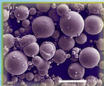
Surface morphology of \text{Al}_{78}\text{Mg}_{20}\text{Zr}_2 powder (a) and cross-section (b) morphology
